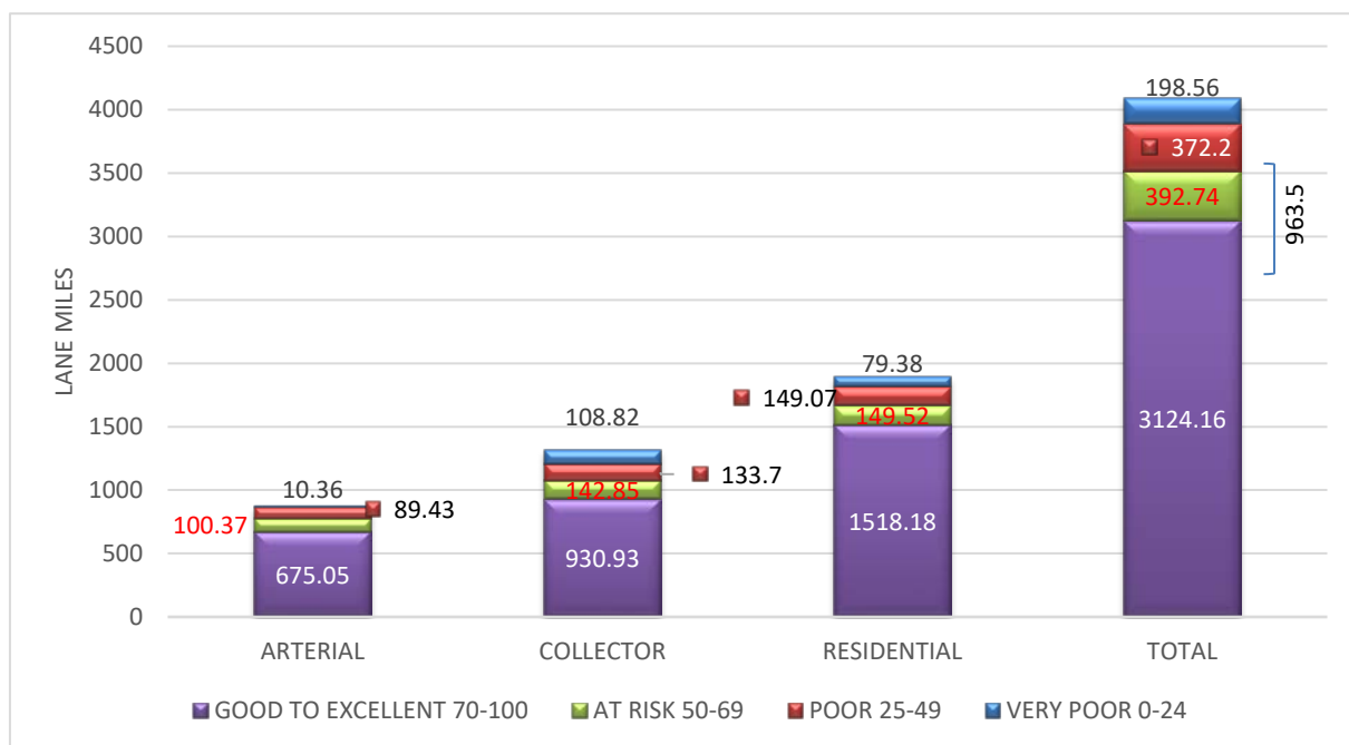
Figure ES.3. Pavement Condition by Category (FY 20/21) – Countywide
