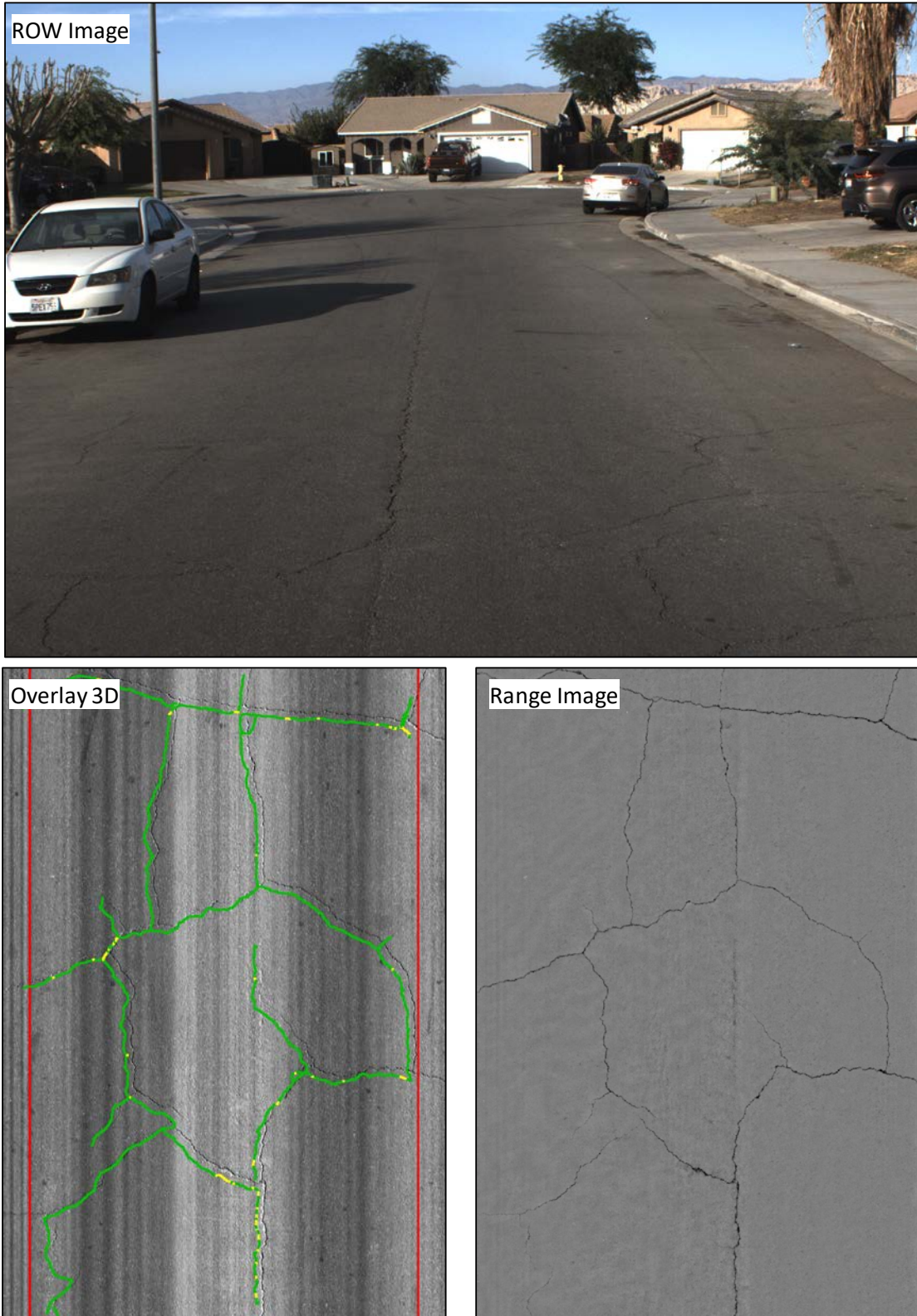
Figure 10D. PCI=68 (At Risk Condition)
