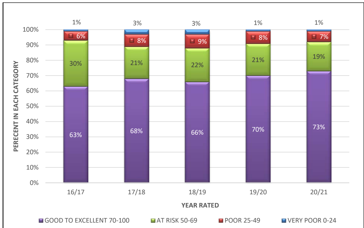
Figure 11. Pavement Condition Trend (Countywide)
