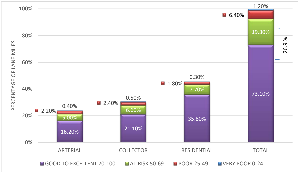
Figure ES.2. Pavement Condition by Category (FY 20/21) – Countywide
