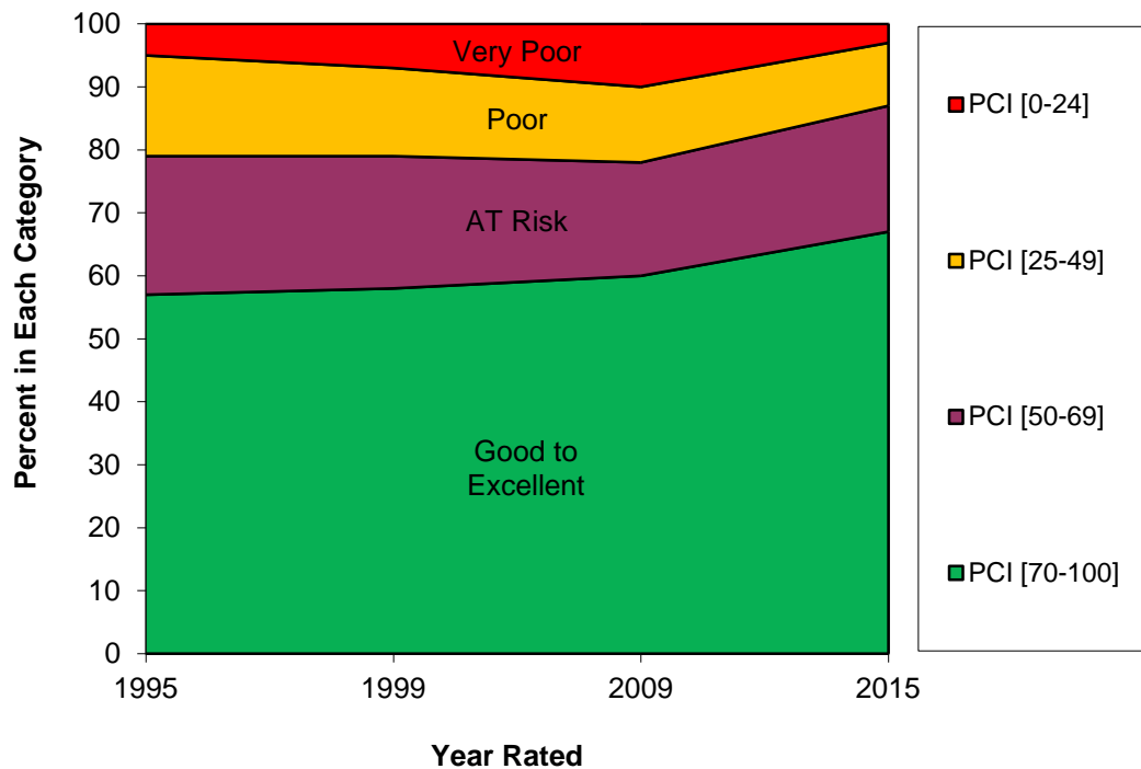
Figure 1. Pavement Condition Trendline (Countywide)
