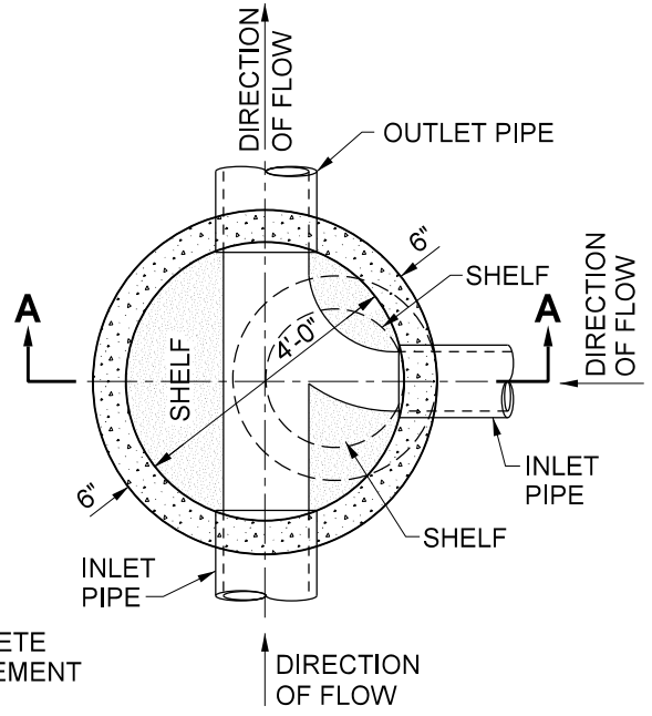
PLAN SECTION
