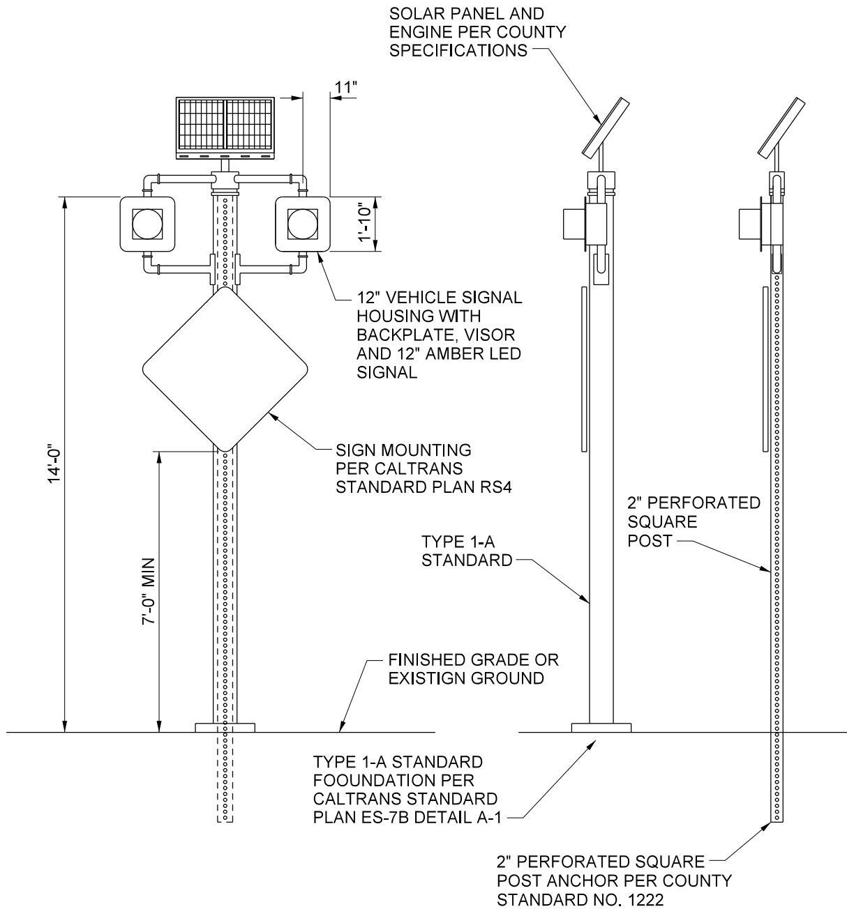
FRONT VIEW
